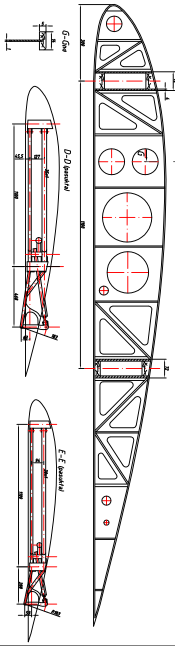
Sparno profilis CLARK-Y
